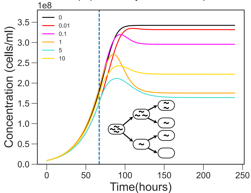
Simulated M1 population dynamics with split inheritance
