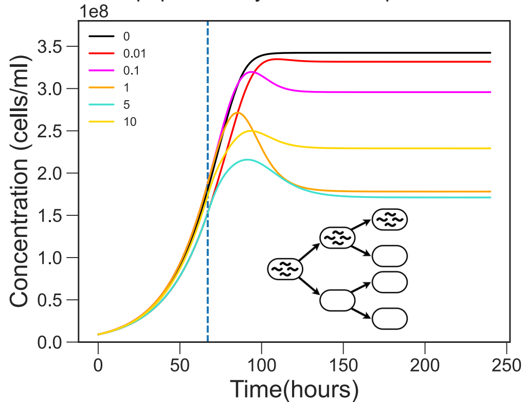
Simulated M1 population dynamics with prioritized inheritance
